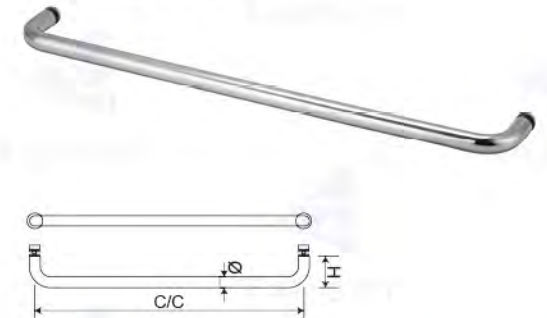
Art. No. DH-800NB Single-Sided Towel Bar
