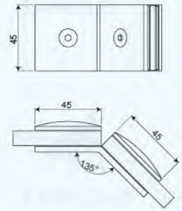
Art. No. GC135-D2 Glass to Glass Double Sided 135° Fixed Bracket
