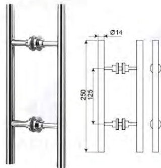
Art. No. DH-01SR "H" Shape Handle
