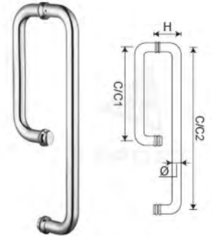
Art. No. DH-801 Pull Handle / Towel Bar Combination
