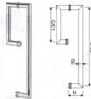
Art. No. DH-804 Pull Handle / Towel Bar Combination
