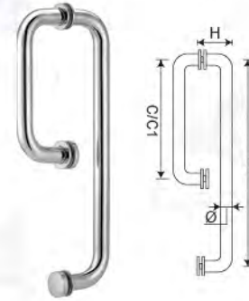
Art. No. DH-801C Pull Handle / Towel Bar Combination with Washers
