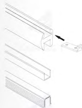
Art. No. SL-101-S U channel
