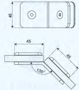
Art. No. GC135-C2 Glass to Glass Double Sided 135° Fixed Bracket
