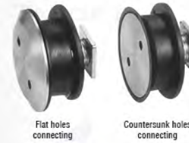
Art. No. SL-007 Fixed Clamp (track to glass)
