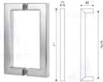
Art. No. DH-14S Double Pull Handle
