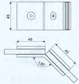
Art. No. GC135-B2 Glass to Glass Double Sided 135° Fixed Bracket
