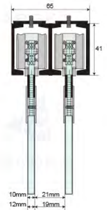
Art. No. SL-012
