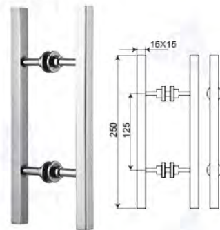
Art. No. DH-01SQ "H" Shape Handle
