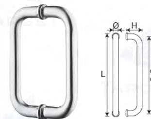
Art. No. DH-207 Double "D" Pull Handle
