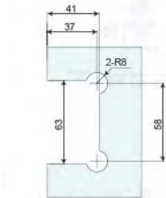
Top or Bottom Mount
