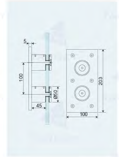
Art. No. OF-H-21 Round Double-Point Support System for Glass Railing
