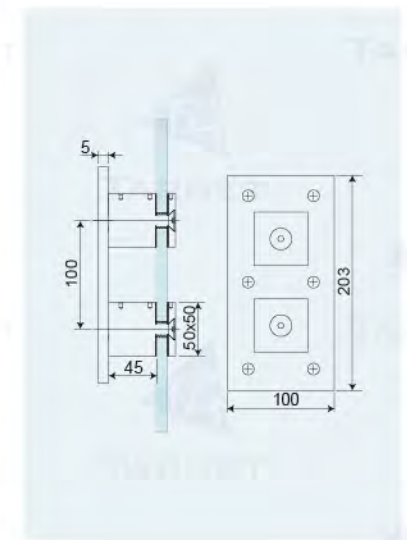
Art. No. OF-H-22 Square Double-Point Mounting Bracket for Glass Railing
