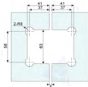
Glass-to-Fixed Transom Mount
