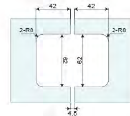
Glass to Glass 180°
