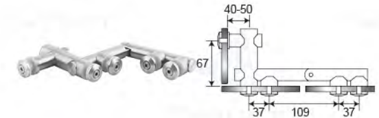
Art. No. WP-21 Angle Door Hinge
