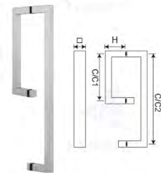
Art. No. DH-801S Pull Handle / Towel Bar Combination
