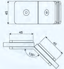
Art. No. GC135-A2 Glass to Glass Double Sided 135° Fixed Bracket
