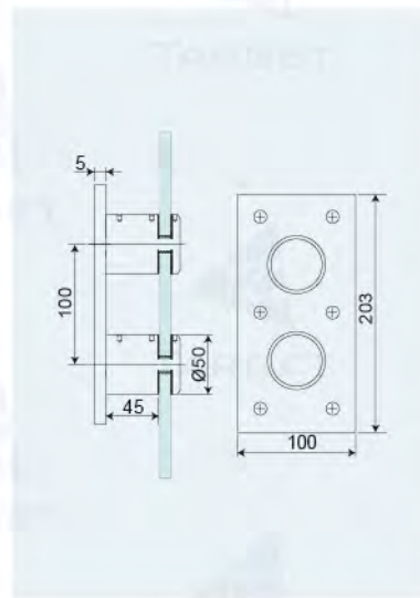
Art. No. OF-H-25 Round Double-Point Mounting Support System for Glass Railing
