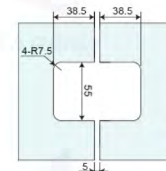
Glass-to-Fixed Transom Mount
